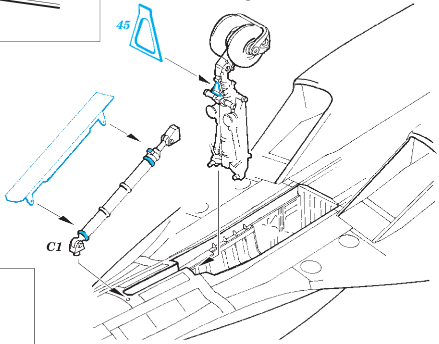
nose undercarriage
