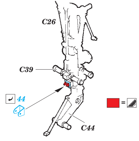
nose undercarriage
